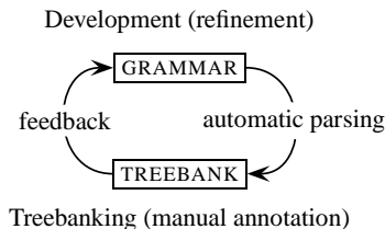
Figure 1: Treebanking Cycles
