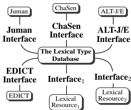
Figure 5: Synthesis of Lexical Resources
